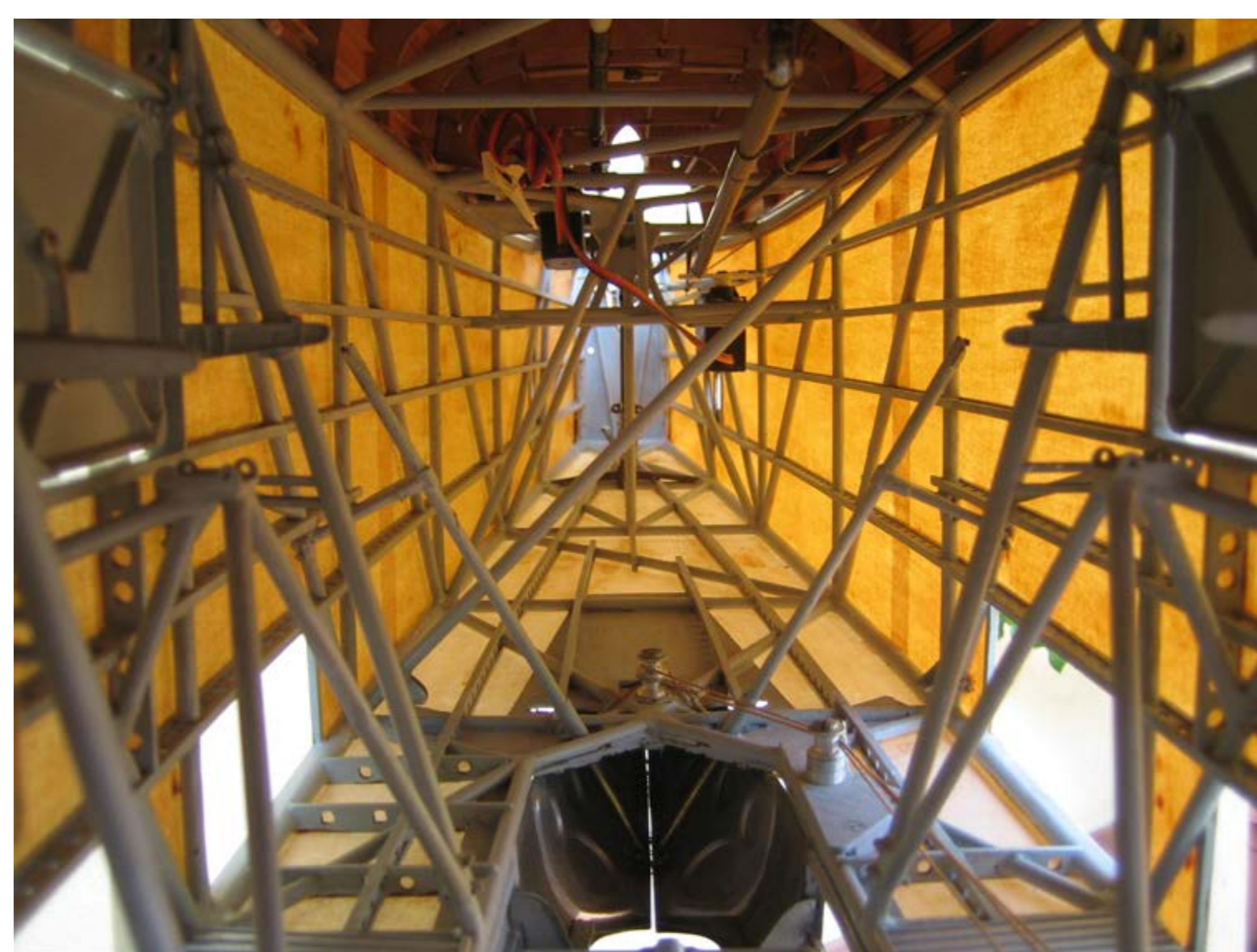
INSIDE OF THE FUSELGE
